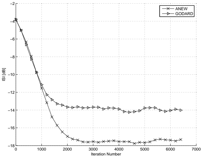
Fig. 27. A comparison between Godard and ANEW algorithms for the 16QAM source going through Channel 4. The averaged results were obtained in 100 Monte Carlo trials. The equalizer's tap length was set to 13, the step-size parameter for Godard and ANEW were set to \mu_G = 0.00008 and \mu_A = 0.00006 respectively, SNR was set to 10 dB. The gain \alpha for ANEW equalizer was set to 1.
