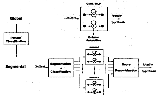
Fig. 2 Global and segmental speaker verification system.
