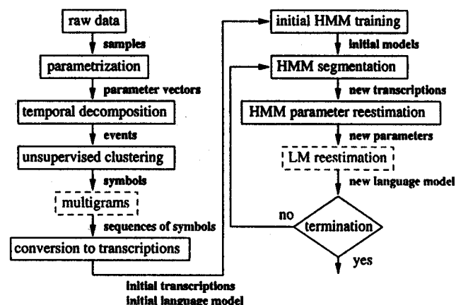
Fig. 1 Data-driven derivation of coding unit set in VLBR phonetic vocoder
